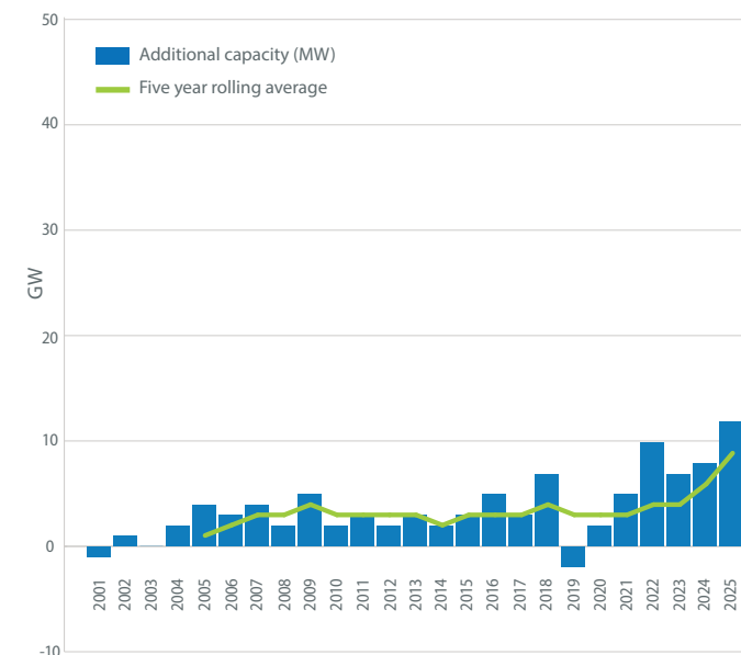
Pumped storage annual additions and five-year rolling average
