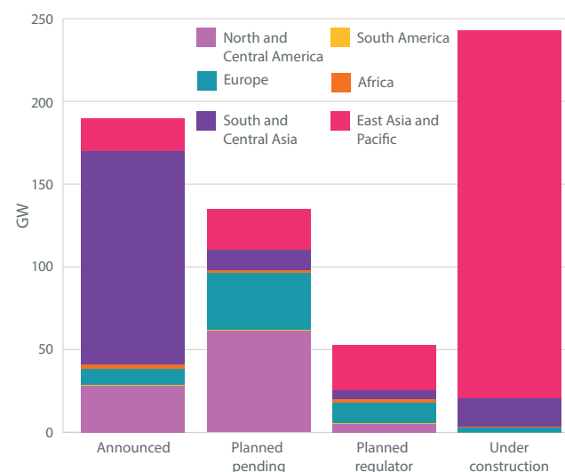
Pumped storage capacity pipeline
