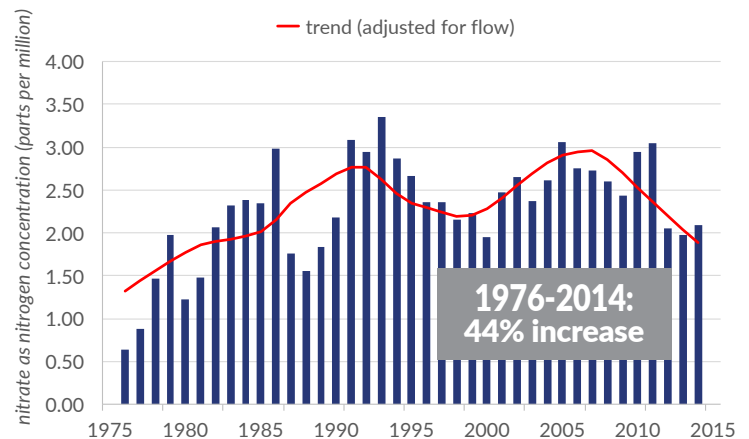
Figure 3. Average annual nitrate concentrations at Hastings Dam, 1976-2014
