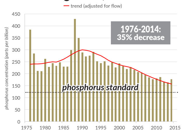
Figure 4. Average summer phosphorus concentrations at Hastings Dam, 1976-2014
