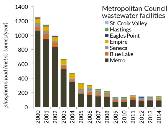
Figure 2. Annual Metropolitan Council wastewater phosphorus loads
