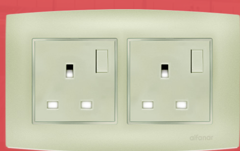
Model: BW4N212224 Type: 13A Double DP -7x14
